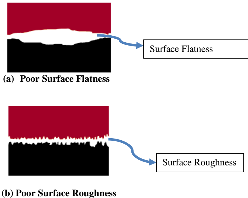
Figure 1: Thermal air resistance due to (a) poor surface flatness and (b) surface roughness (courtesy: Dr. Miksa de Sorgo 4 , Electronics Cooling, 2000)
