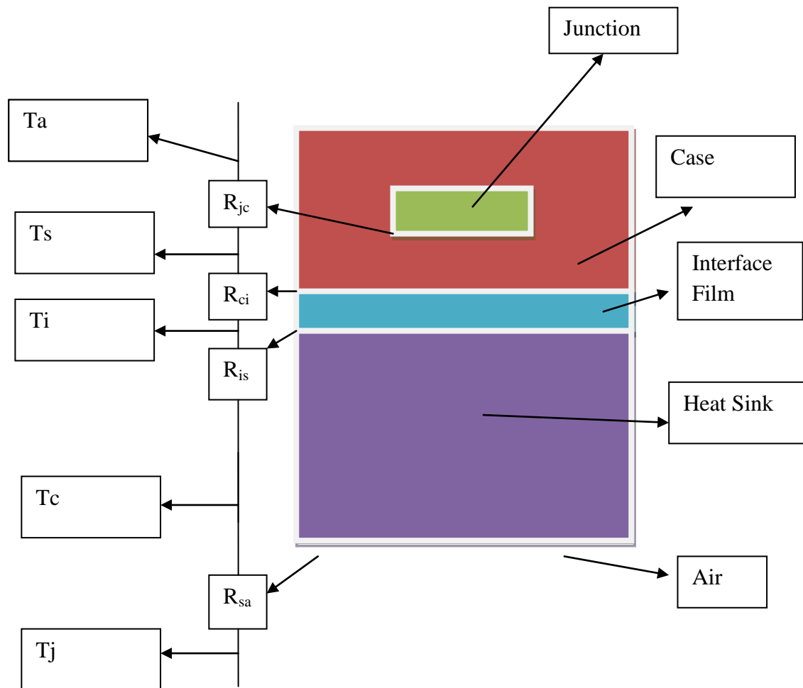
Figure 2: Thermal resistance diagram of the PCB assembly
