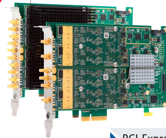
8-channel-versions and high-voltage versions occupy 2 slots width
