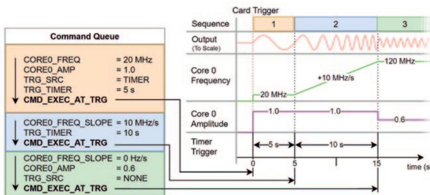
In DDS-mode, only a few commands are needed to e.g. generate a sine wave (orange block), increase the frequency (blue block) and lower the amplitude (green block).
