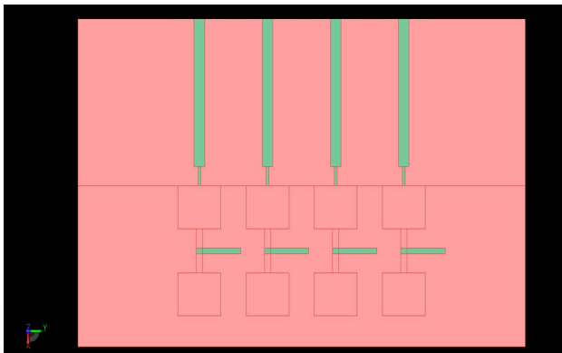
Figure 1: Shown is a top view of the antenna array with the substrate layers shown in red and the metal feed lines and parasitic elements in green. The patches are shown as outlines because they are covered by a second substrate layer.
