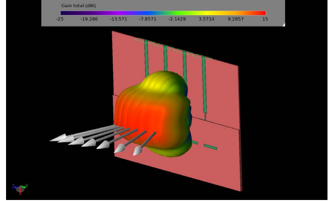
Figure 7: Sweeping the phase shift from -90 to 90 degrees in 30 degree increments generates seven beams that cover a broad area.
