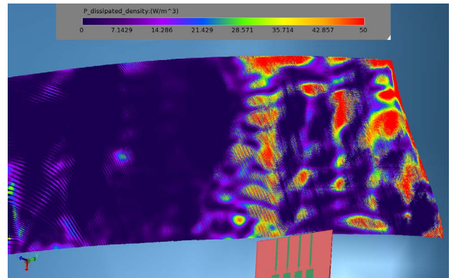
Figure 13: The dissipated power on the surface of the head phantom from the radiating array is computed by the software and displayed.
