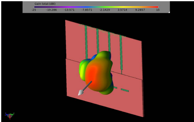
Figure 6: With a phase shift of 90 degrees between the antenna elements the beam shifts about 30 degrees to the side.
