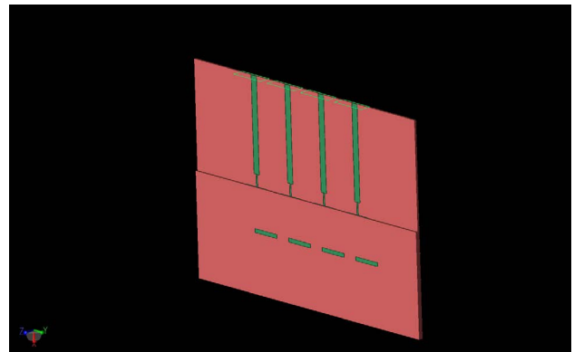
Figure 2: The antenna array is shown in three dimensions with the edge of the top substrate layer more visible over the patches. The four nodal waveguide feed ports are visible on the top of the array.
