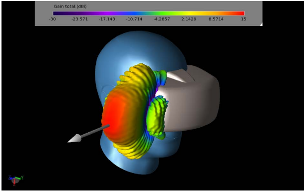
Figure 10: The computed gain pattern for the case of all elements in phase is shown with a strong gain of nearly 15 dBi and a fan-shaped beam.
