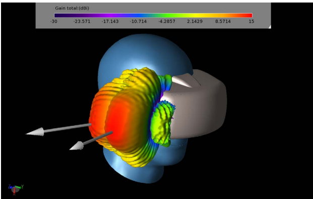
Figure 12: Both beams with 0- and 90-degree phase shifts are shown in this image.
