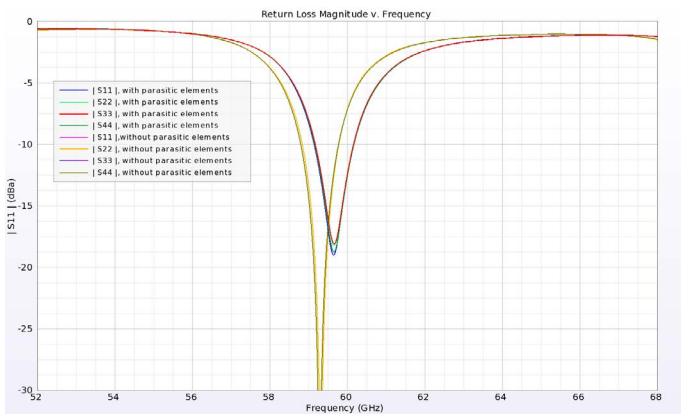
Figure 3: The return loss for each element of the array is quite similar. The addition of the parasitic element shifts the response higher in frequency and reduces the null depth.
