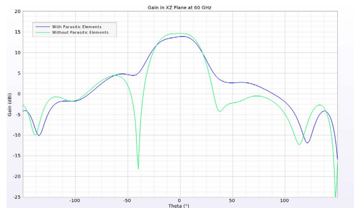
Figure 4: The gain pattern broadside of the array is fairly wide with the parasitic elements included. Without the parasitic elements there are undesired nulls present in the pattern.
