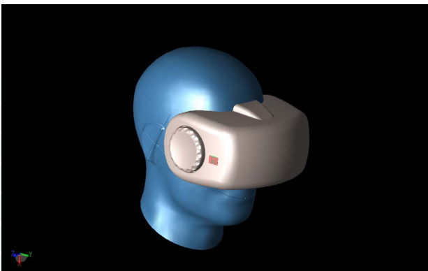
Figure 8: The antenna array is shown mounted on a virtual reality headset. The headset is attached to a phantom head model.
