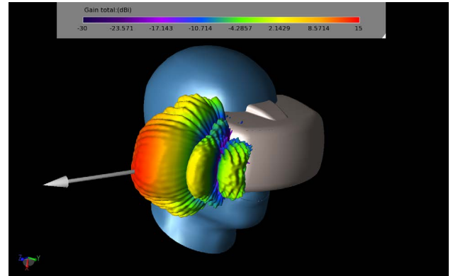
Figure 11: After applying a 90-degree phase shift between the elements the beam is shifted about 30 degrees to the side.
