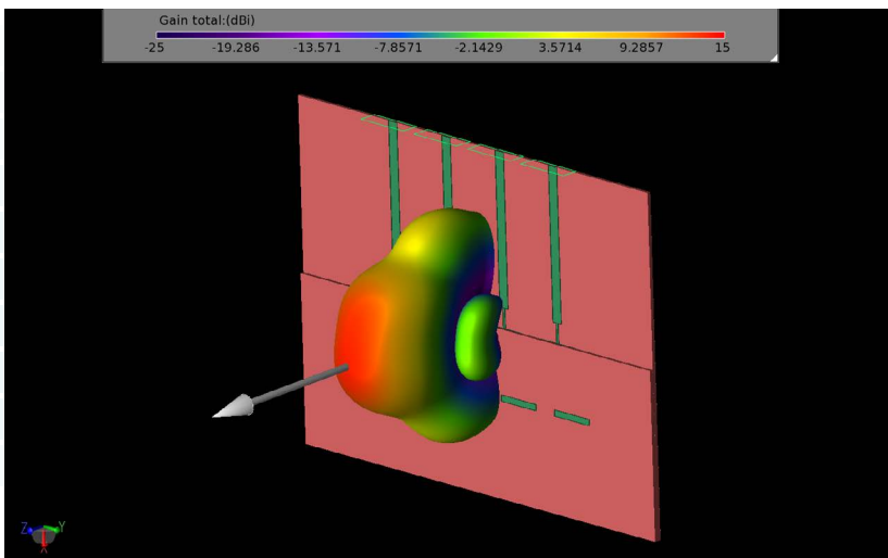
Figure 5: The three-dimensional gain pattern for the equal phase case shows peak gain to the side with a fan shaped pattern.
