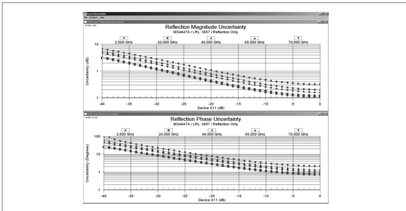
Figure 12. Reflection ( S_{11} ) Uncertainty Curves.
