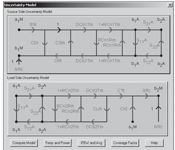
Figure 4. Flow Graph Representation of Model.
