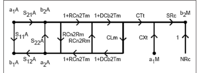
Figure A2. Load Side Uncertainty Model.
