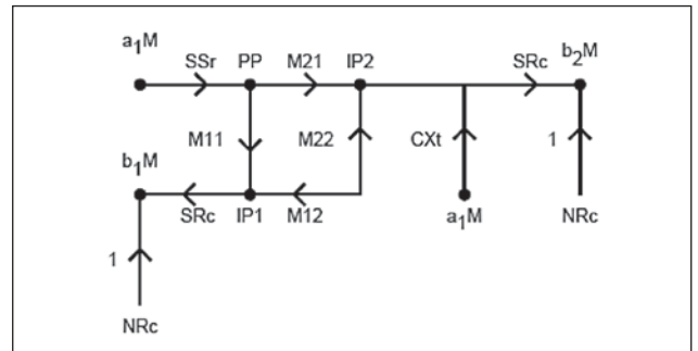
Figure A3. Condensed Uncertainty Model.
