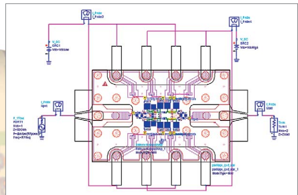
Co-simulation with Layout Components allows you to incorporate layout artwork in the schematic environment to enable concurrent analysis of circuit performance along with critical physical effects.
