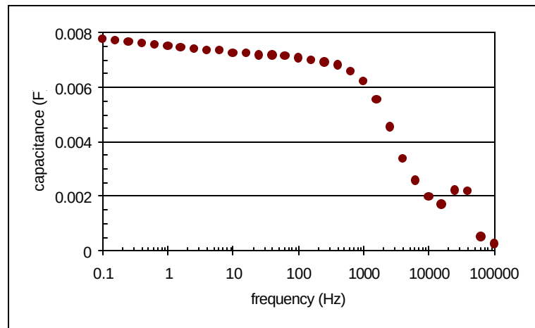
Figure 6. Capacitance vs. frequency.
