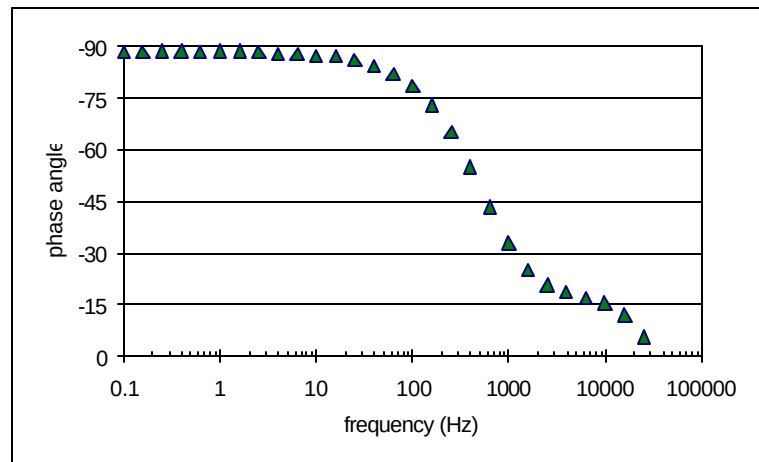
Figure 7. Phase angle vs. frequency.
