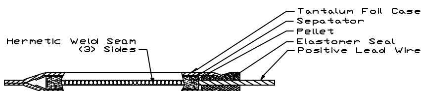
Figure 2. Drawing of the prototype capacitor showing a partial cut-away view. The overall dimensions are 19mm X 18mm X 1.4mm.
