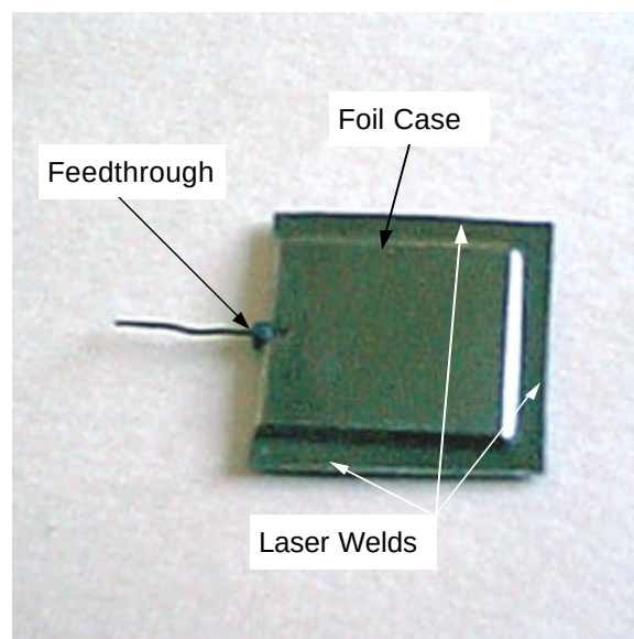
Figure 4. Photograph of the prototype tantalum Hybrid capacitor. This particular unit has a capacitance of 8mF at a rating of 5.5 volts. The case is only 1.4 mm thick.
