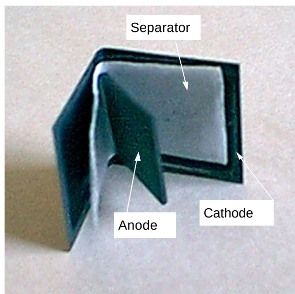
Figure 3. Photograph of a disassembled prototype tantalum Hybrid capacitor showing the cathode coating, anode pellet, and separator. The case is partially unfolded to show interior.
