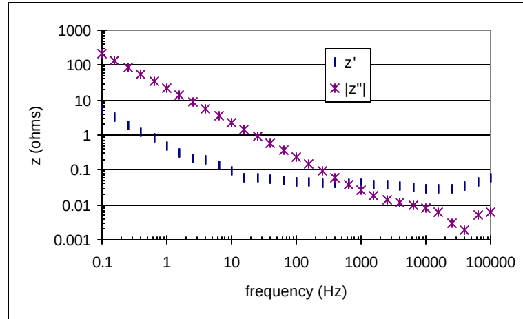
Figure 5. Resistance and reactance vs. frequency in the range of 0.01Hz to 50kHz.
