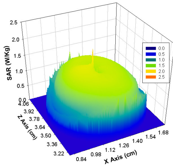
Figure 4: Distribution of the SAR in W/kg in the region containing the biological cells. Here the biological cells were assumed to be evenly distributed over the entire glass fiber filter. Results are from XFDTD for an input power of 0.5 W into the waveguide and a frequency of 1 GHz, and are imported into SigmaPlot for plotting and analysis.
