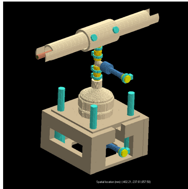
Figure 3: Numerical mesh of the cell perfusion apparatus created by XFDTD.
