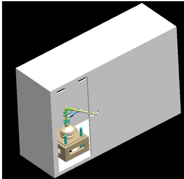
Figure 1: Geometry of the cell perfusion apparatus within the waveguide as created in Solid Works and imported into XFDTD.
