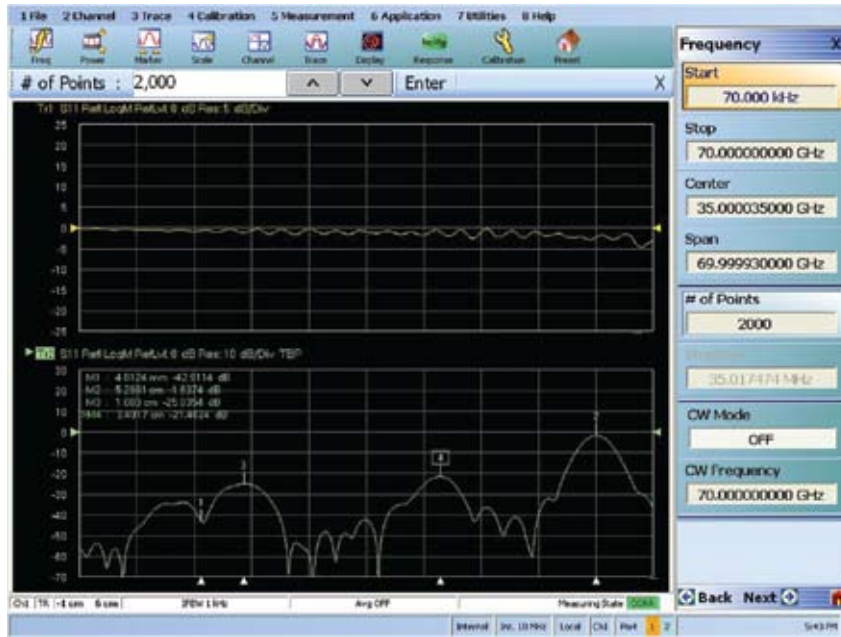
Figure 1. Time and Frequency Response of a Microstrip Circuit
