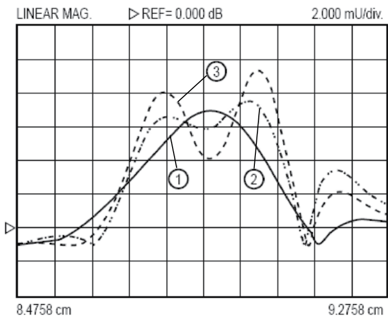
Figure 3. Wide bandwidth provides improved discontinuity resolution
