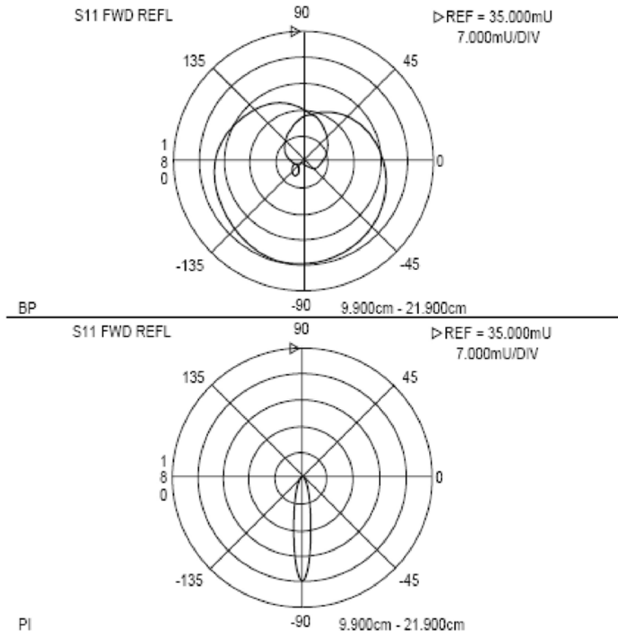
Figure 10. Normal Bandpass display and the Phasor Impulse display of waveguide
