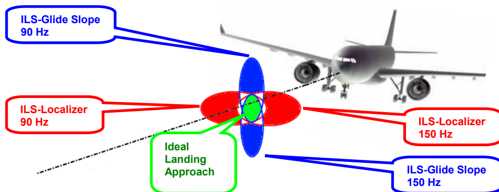
Figure 5: Approach navigation using instrument landing system (ILS)
