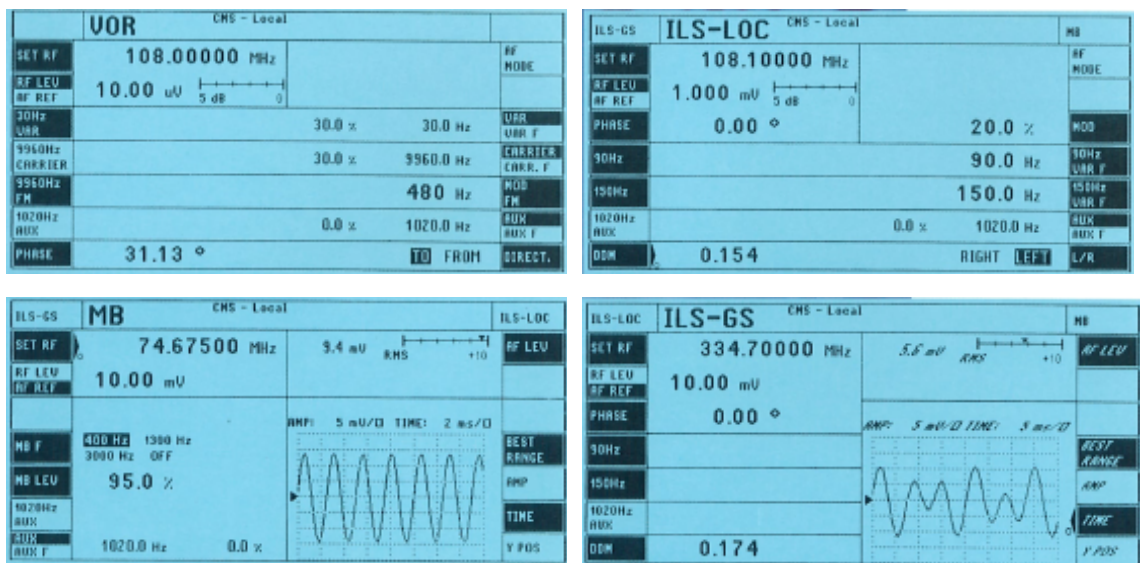
Figure 43: R&S ® CMS57 generation and analysis of VOR, ILS, and MB signals
