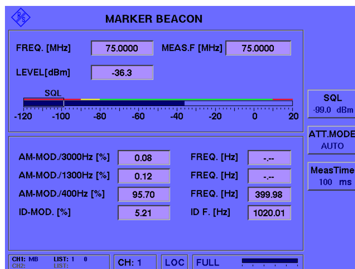
Figure 34: R&S®EVS300 marker beacon with AF audio output and squelch
