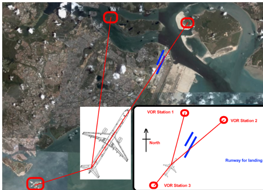
Figure 6: Final descent approach localization using VOR stations
