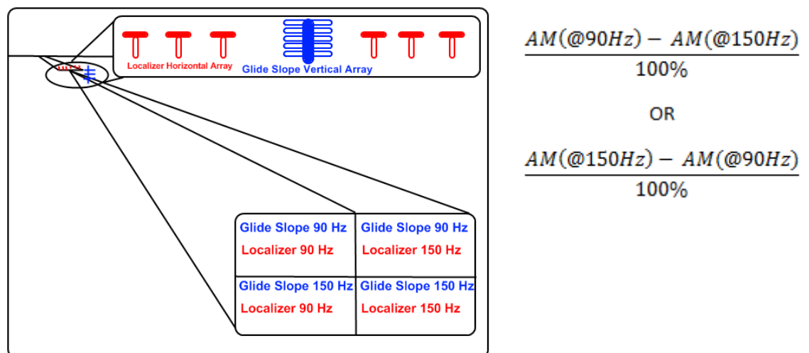
Figure 9: ILS 90 Hz and 150 Hz convention
