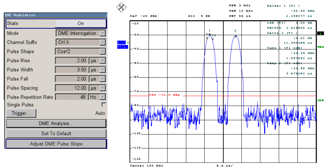
Figure 23: R&S® SMA-K26: DME generation and time-domain pulse width analysis using the R&S® FSQ
