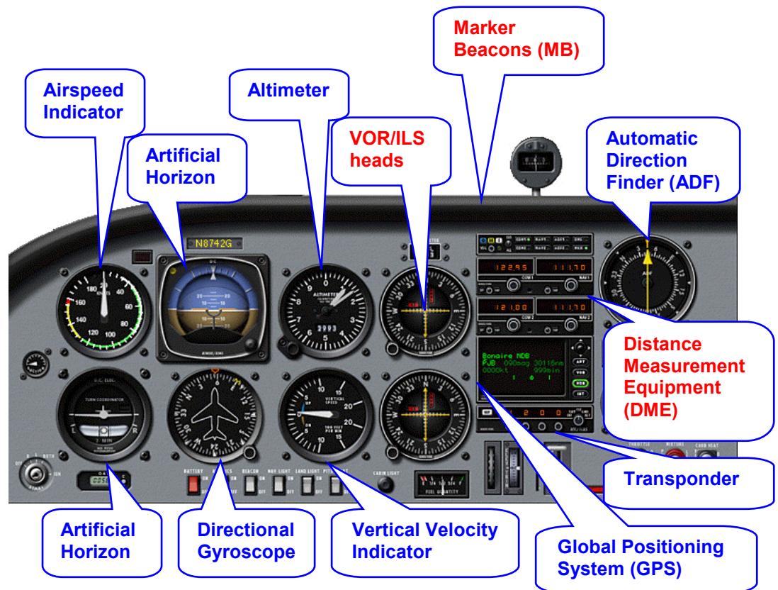
Figure 2: Cockpit view of various navigation, landing, and DME instrumentation
