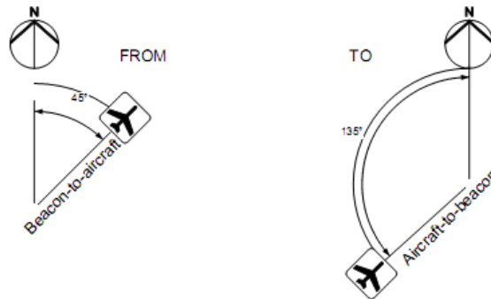
Figure 7: FROM and TO bearing angle conventions
