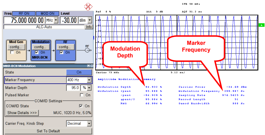
Figure 20: R&S ® SMA-K25: MB AM modulation settings are shown. A modulation depth of 95 % at 75 MHz carrier frequency is set. The modulation depth at carrier frequency is illustrated using the R&S ® FS-K7 analog demodulation.
