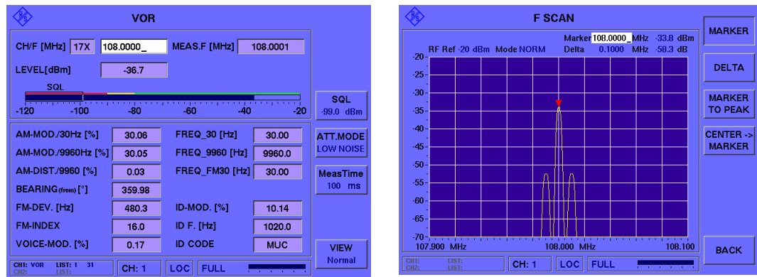
Figure 29: R&S®EVS300 VOR analysis and R&S®EVS-K1 FSCAN option displaying the RF spectrum
