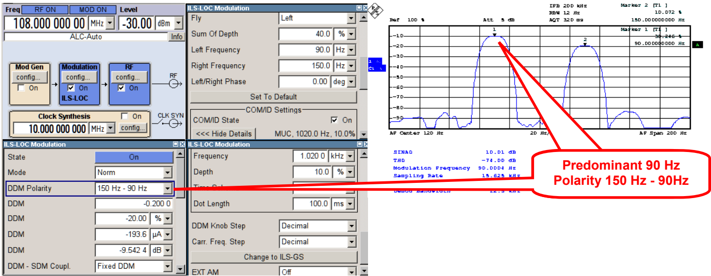
Figure 19: R&S ® SMA-K25: The ILS-LOC modulation parameter settings are shown. The ILS-LOC AM 90 Hz - 150 Hz spectrum is illustrated using the R&S ® FS-K7 analog demodulation (notice the flexibility in the DDM polarity).
