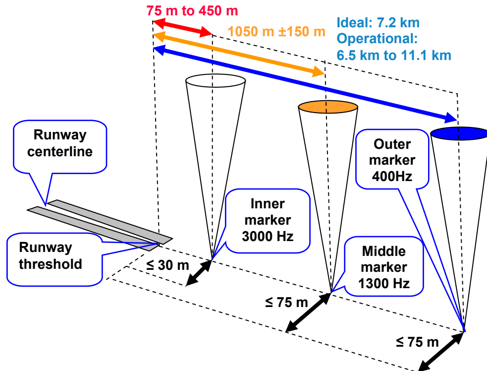
Figure 14: Marker beacon placement with respect to runway
