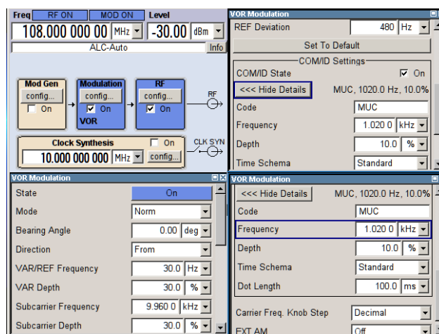
Figure 16: R&S ® SMA-K25: VOR option is activated in the MODULATION section.
