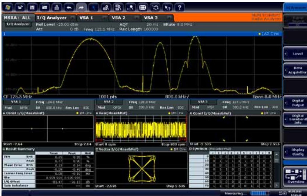
Multi-standard radio analyzer (MSRA): Signals are captured once, then analyzed to different standards and at different frequencies in parallel.
