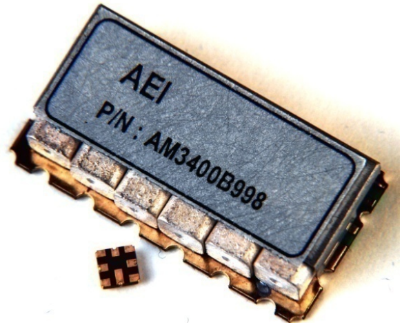
Figure 7 – SAW filter compared to ceramic filter
