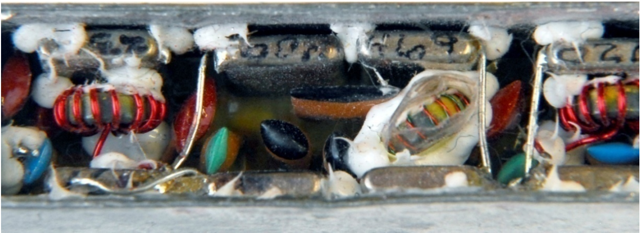
Figure 8 – Inside a crystal filter
