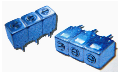
Figure 9 - Helical filters
