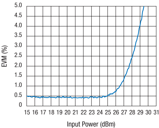
Figure 3. SKY13385-460LF SOI SP3T Switch 802.11g EVM
