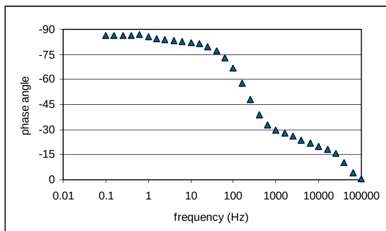
Figure 6. Phase angle vs. frequency for THQA2016502. The capacitor has a phase angle of -45° at a frequency of 275Hz. At lower frequencies, the phase angle rapidly approaches -90°.
