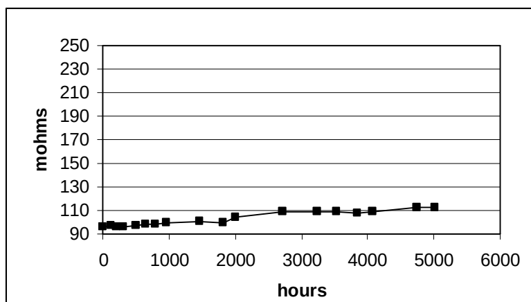
Figure 10. ESR (1kHz) vs. time for THQA2016502 capacitors with 2X the original cathode. This test is running at 16 volts and 85°C. The resistance has increased gradually since the beginning of the test.
