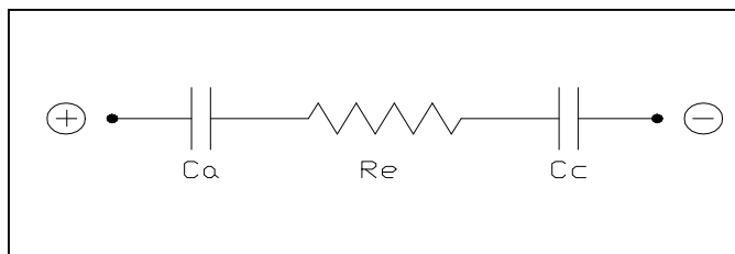
Figure 1. Electrical schematic of an electrolytic capacitor. The individual positive and negative electrode capacitances are connected in series by the electrolyte.
