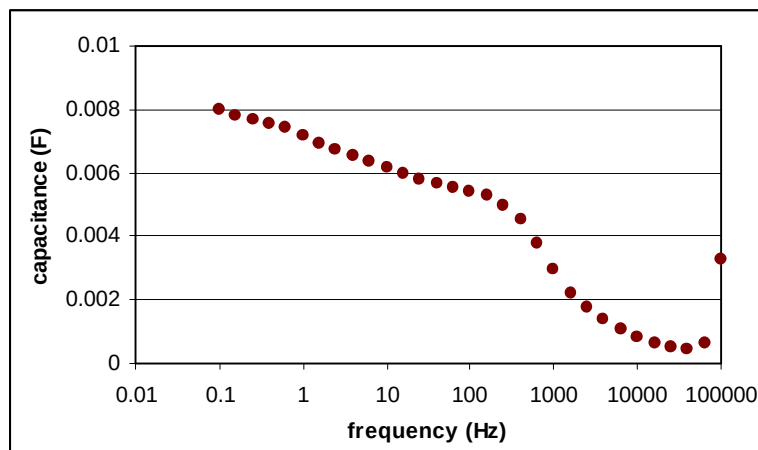
Figure 4. Capacitance vs. frequency for THQA2016502. The capacitance is 5.2mF at 120Hz.
