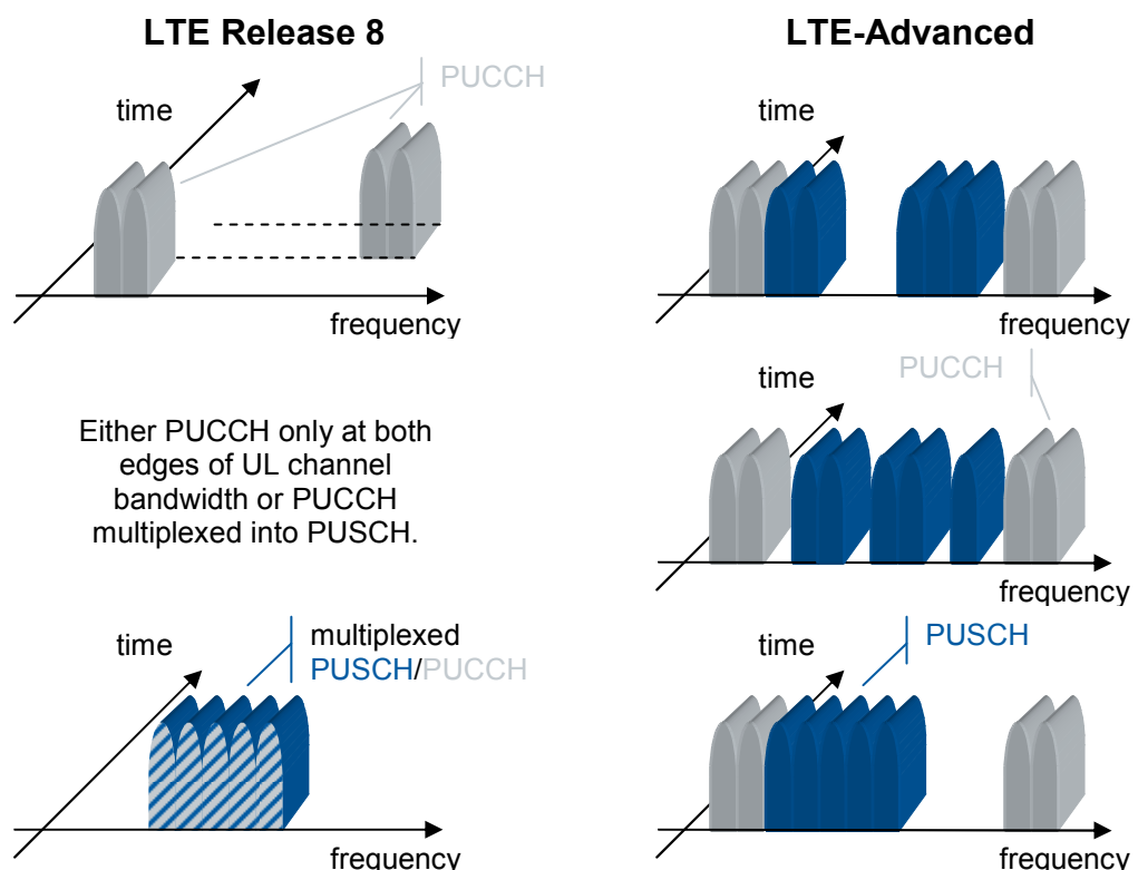
Figure 7: LTE Release 8 and LTE-Advanced uplink transmission schemes
