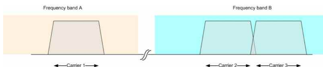
Figure 2: LTE-Advanced non-contiguous spectrum deployment
