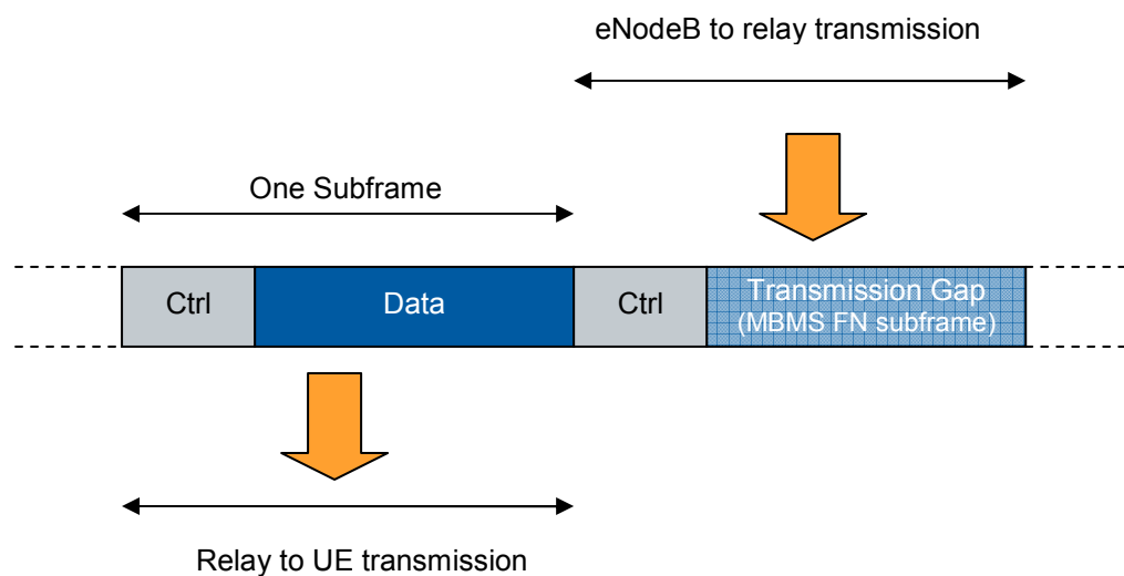
Figure 13: Example of relay-to-UE communication using normal subframes (left) and eNodeB-to-relay communication using MBSFN subframes (right)
