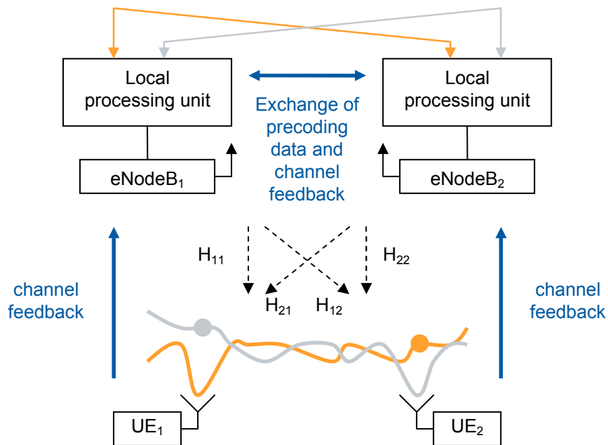
Figure 10: Principle of CoMP processing in a distributed approach between two eNodeBs
