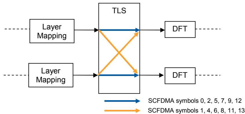
Figure 6: LTE-Advanced time domain layer shifting in uplink
