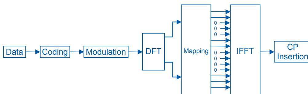
Figure 8: Block diagram for clustered SC-FDMA in uplink LTE-Advanced
