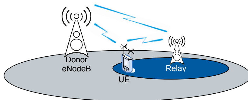
Figure 12: Type 2 relay station
