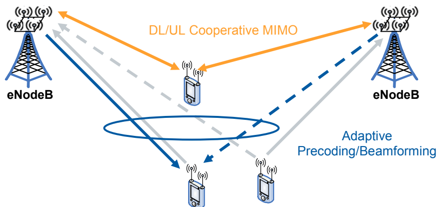
Figure 9: Principle of CoMP
